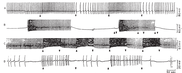
Fig. 2. Effect of photostimulation on neurons A, B, C, and D from Fig. 1. Light on and off at arrows. Note the discontinuity in record B, where a 300 sec period of recording was cut out between the brackets.
