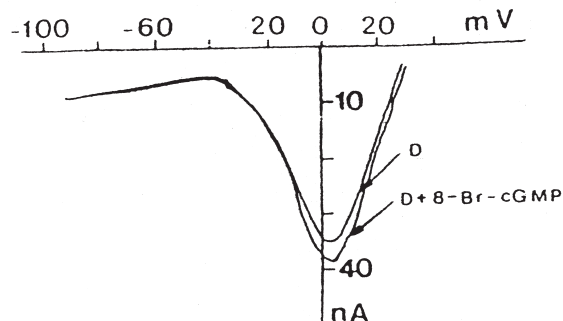
Fig. 16. Ramp-generated I - V curve from -100 mV holding potential in Ba^{2+} /TRIS/TEA/4-AP solution in the absence of 8-Br-cGMP and 10 min after it was adding to the bathing solution/dark.
