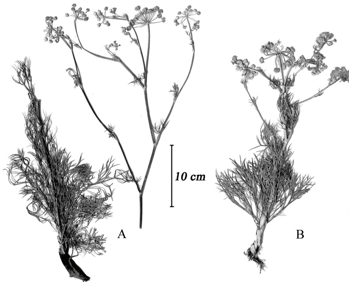
Fig. 3. Herbarium specimens of the facultative serpentinophyte Seseli rigidum from serpentine (A) and calcareous (B) soil.
