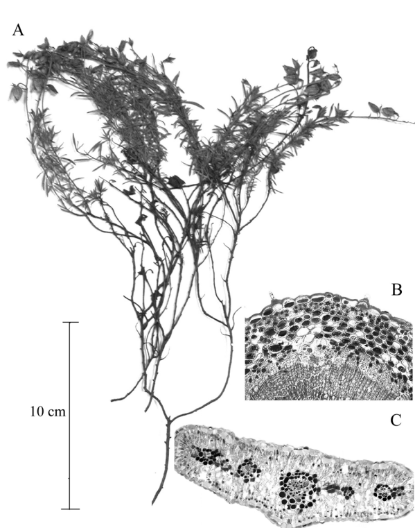
Fig. 1. Herbarium specimen of the obligate serpentinophyte Fumana bonapartei (A) and cross section of the stem (B) and leaf (C) with noticeable presence of “vague” contents in parenchymatous cells.
