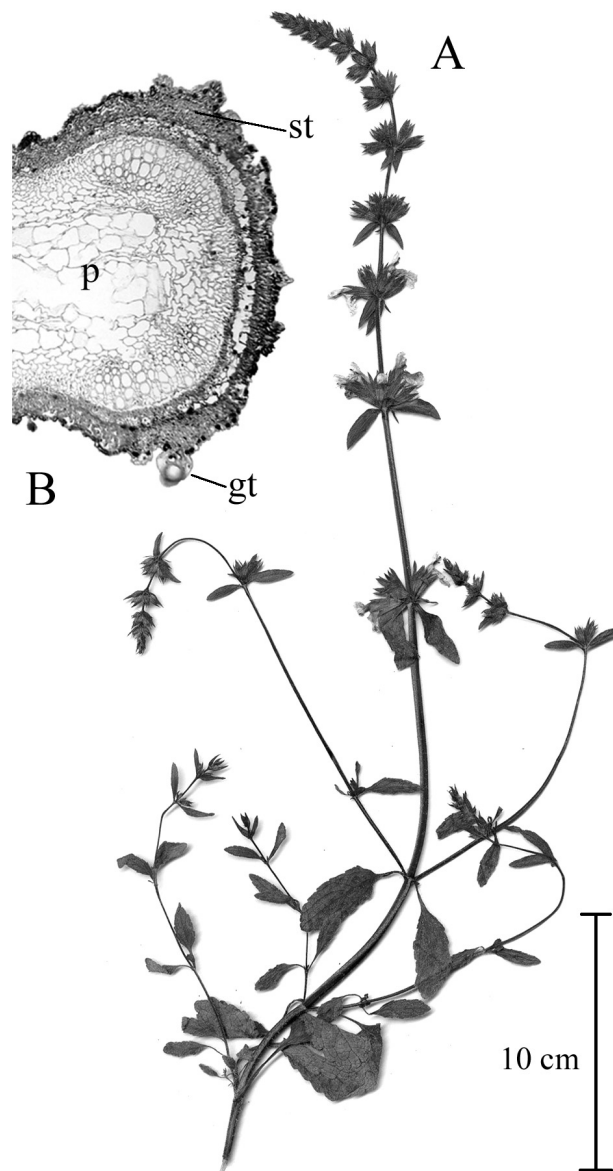
Fig. 2. Herbarium specimen of the obligate serpentinophyte Stachys recta var. chrysophaea (A) and part of a cross section of the stem (B). p – pith, st - sclerenchyma tissue forming “clusters” in angles of the squared stem, gt – glandular trichome.
