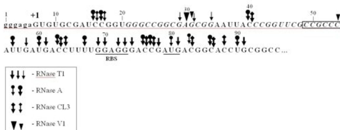
Fig. 2. Secondary structure probing of the sgm mRNA with different RNases. (a) Gel analysis of products obtained by limited cleavage with RNases. Lanes 1 and 9 correspond to in vitro transcribed control mRNA. Lane 2 corresponds to a RNase A ladder generated under denaturing conditions. Lanes 10 and 11 – RNase T1 ladder generated under denaturing conditions. Lanes 18 and 19 – alkaline-hydrolysis ladder (AH) with increasing incubation time. Lane 20 – a 10 bp DNA ladder. Lanes 3-8 and 12-17 correspond to products of limited cleavage with decreased concentrations of the indicated RNases. Vertical arrows and boxed parts of the autoradiogram indicate position of a stem. Horizontal arrow points to digestion with RNase V1. (b) Summary of secondary structure probing of the sgm mRNA with different RNases. The putative regulatory sequence (CCGCCC) is shown in the box. Transcription start site of the sgm gene in M. zionensis is indicated (+1). RBS and the translational start codon are underlined. Major and minor cuts are indicated by thicker and thinner symbols as listed in the separated box. Small letters represent nucleotides from T7 promoter sequence. Letters in italics represent nucleotides predicted to be in a stem.
